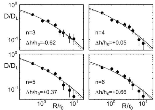
FIGURE 2 The size-dependent diffusion coefficient D of transmembrane inclusions with varying hydrophobic mismatch (symbols) is equally well fitted by Eq. 1 (solid) and Eq. 2 (dashed). Please note that D is normalized by the diffusion coefficient D_L of a single lipid. Since the fitting parameter R_c = h\eta_m/\eta_c takes on too-small values when using Eq. 2 (see also main text), Eq. 1 appears to be the more appropriate fit function.
